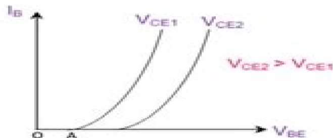
Fig. Input characteristics of CE configuration.
