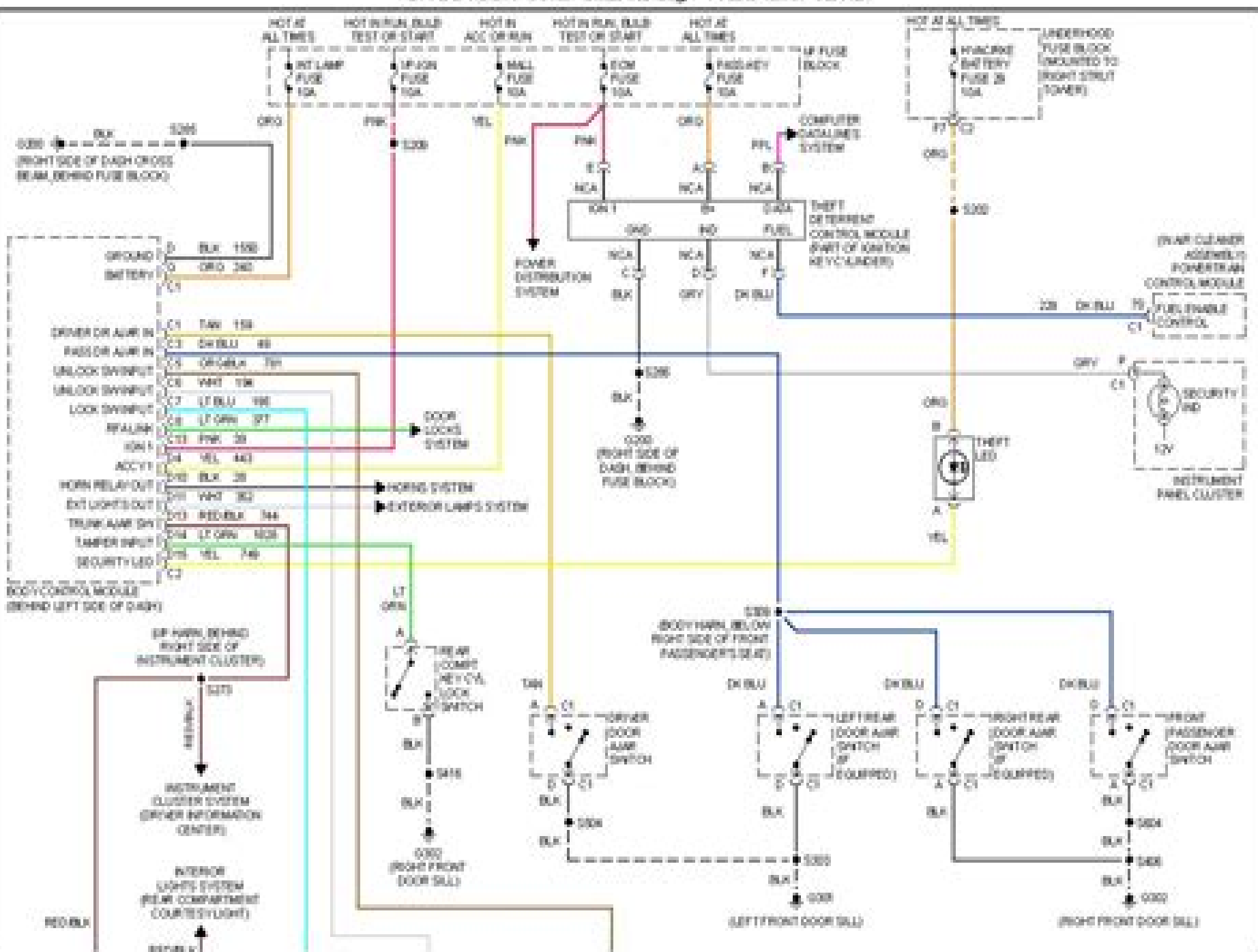
2002 Pontiac Grand Prix SE-Fig. 7: Anti-theft Circuit
