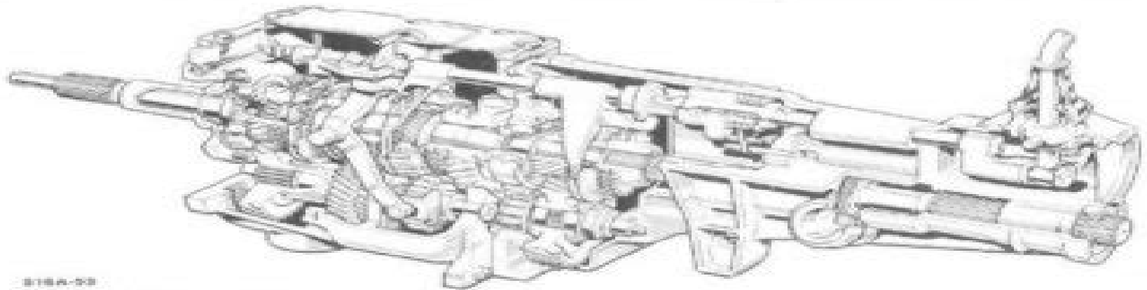
Fig.111. 'N' Transmission.
