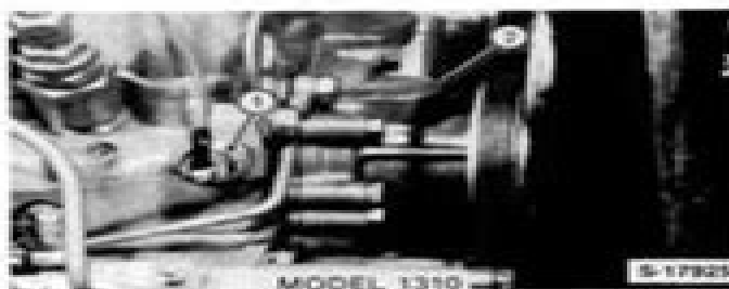
Figure 9 Oil Pressure Switch — Model 1310 1. Sender Switch 2. Water Pump Assembly
