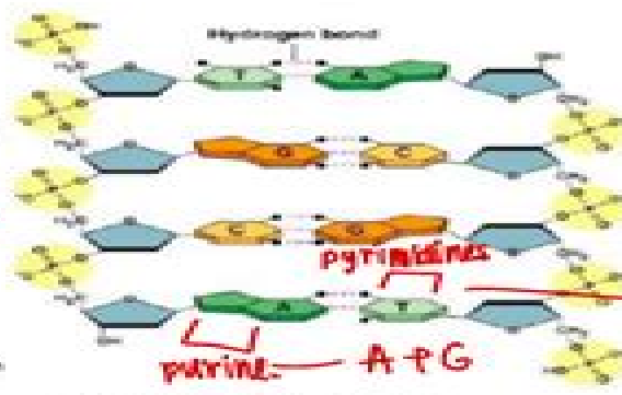
(b) Partial chemical structure
