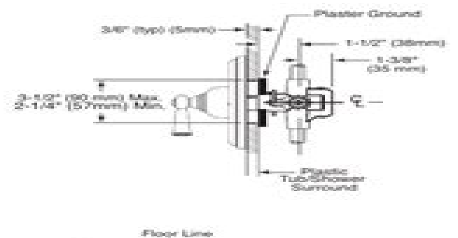
THIN WALL APPLICATION
