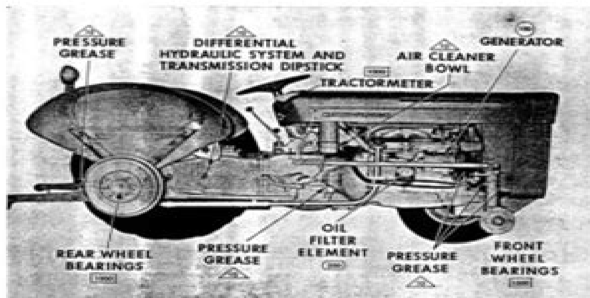
Lubrication Chart
