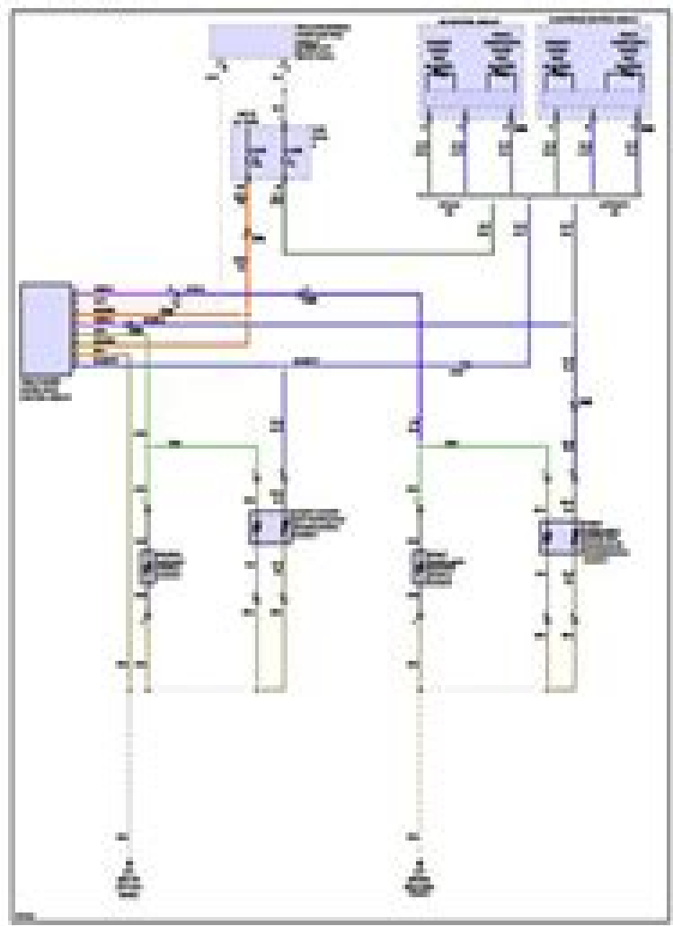
Fig. 1 Heated Seats Circuit
