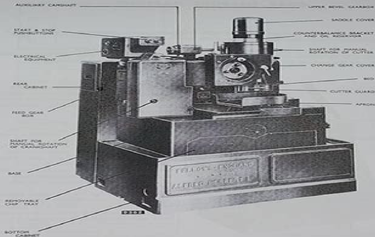
Fig. 1 The Fellows/England Type 7125A Gear-Shaping Machine.
