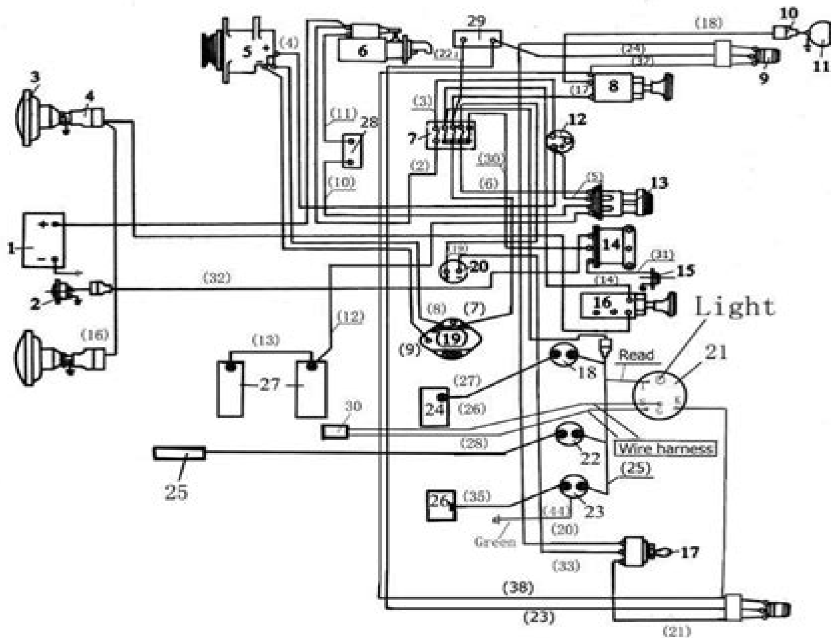
Fig. 6 - 1 Wiring diagram of the electrical system
