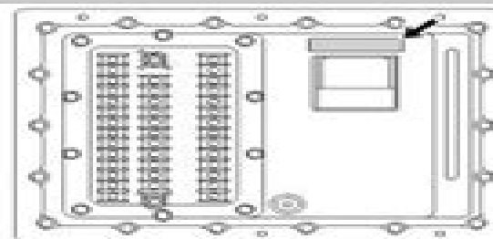
Illustration 6 g00350244 Location Of GSC+P Part Number Rear View Of GSC+P
