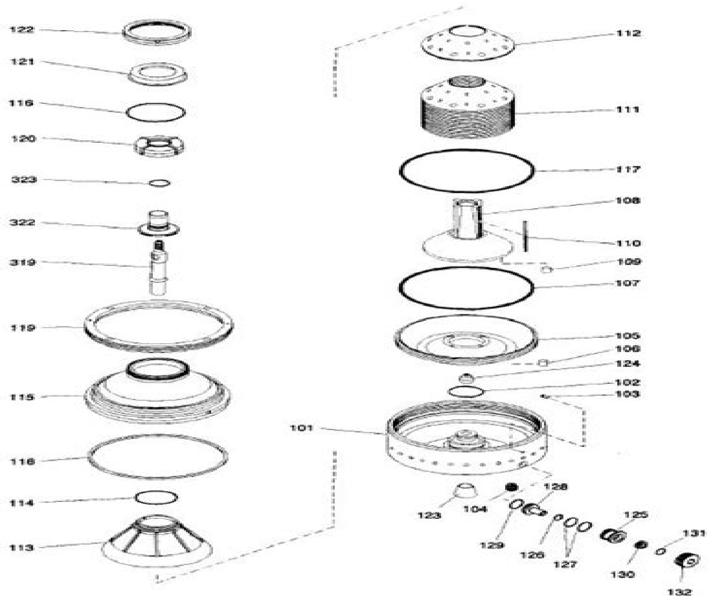
Fig. 2-31 Bowl Assembly Drawing (SJ10F, 15F, 30F) NOTE: FH/FP/SH types are the same as F type.
