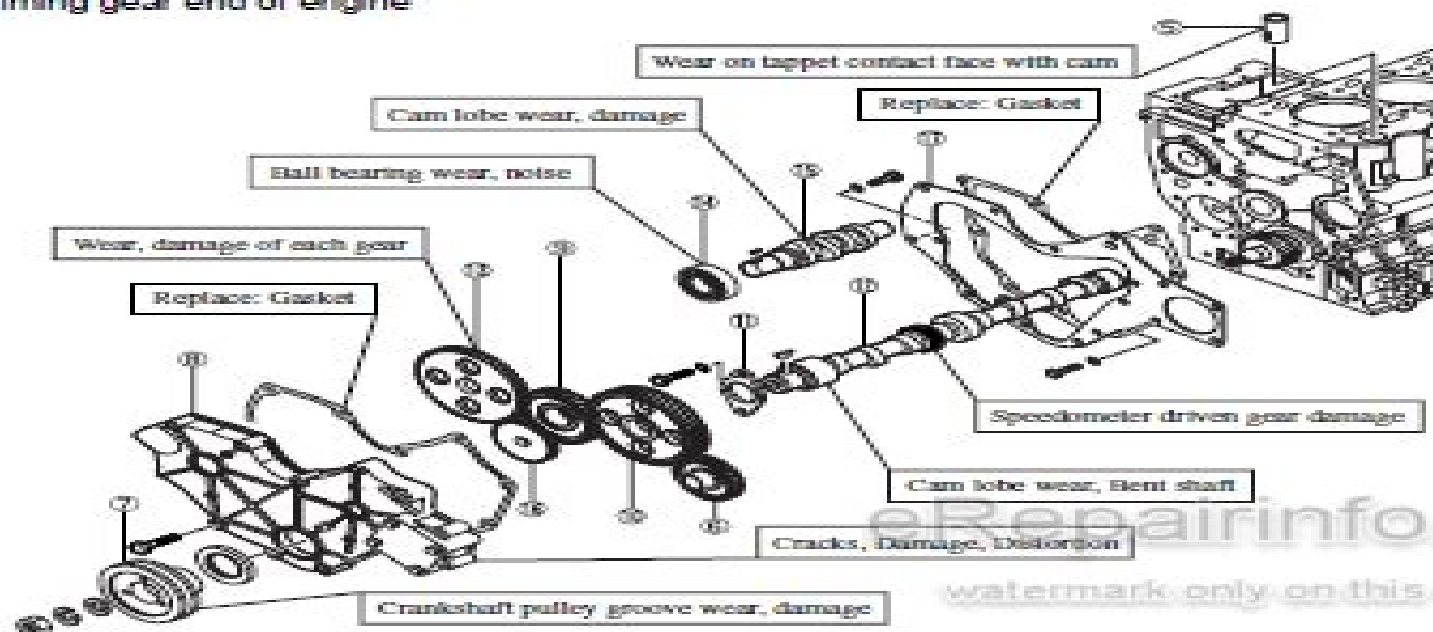
Disassembly of timing gear and camshaft
