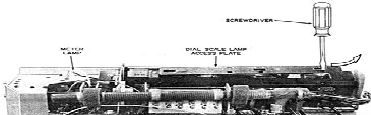
FIGURE 11 – DIAL SCALE LAMP AND METER LAMP REPLACEMENT
