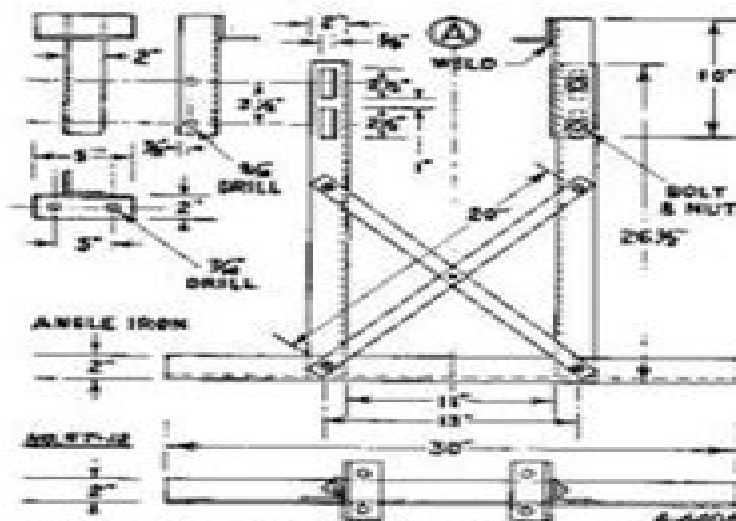
ILLUSTR. 18B. CONSTRUCTION DETAILS OF THE HOME-MADE STAND WHICH SUPPORTS THE FRONT OR ENGINE SECTION.
