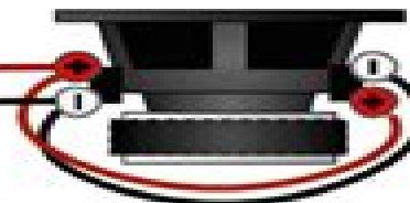
2 x 2 ohm dual voice coil in parallel = 1 ohm
