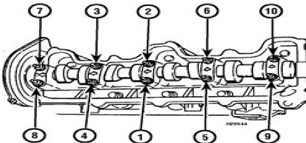
11.16 Camshaft bearing cap tightening sequence
