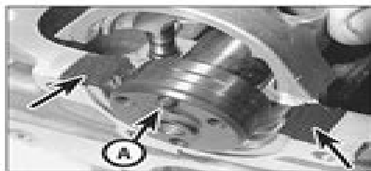
11.14 Apply sealant to the cylinder head mating surface of No 1 camshaft bearing cap (arrowed) then refit the caps ensuring the camshaft locating pin is correctly positioned (A)
