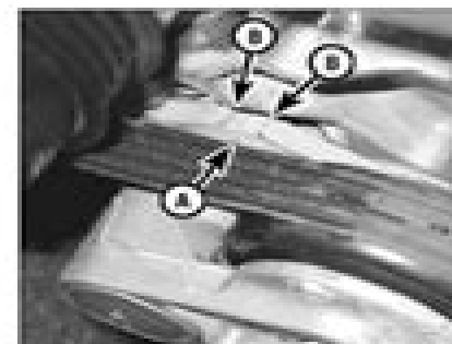
12.4b The tensioner for the air conditioning compressor drivebelt is harder to see. The mark (A) on the moveable part of the tensioner must be within the acceptable range marks (B)
