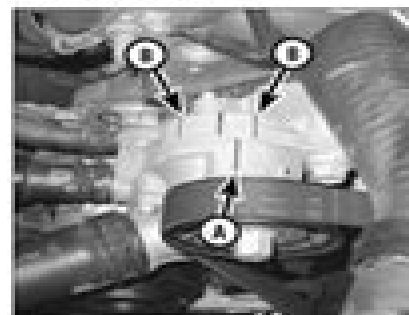
12.4a The mark (A) on the main belt's tensioner must remain between the marks (B) on the tensioner mount (V8 shown, main belt)
