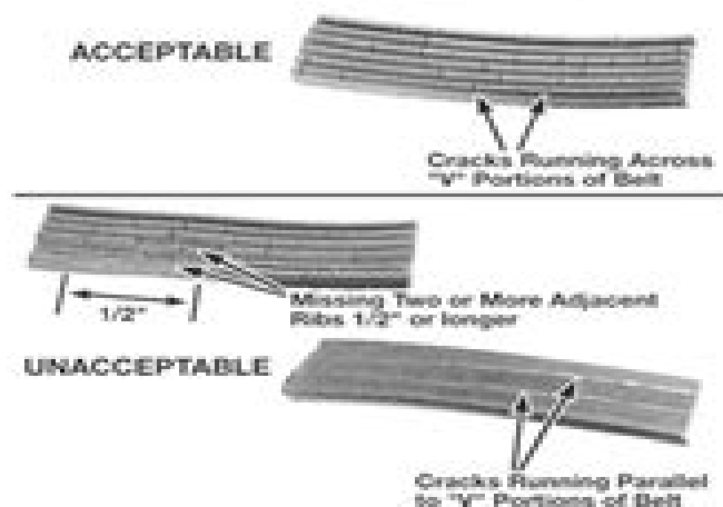
12.2 Check the belts for signs of wear like these - if it looks worn, replace it
