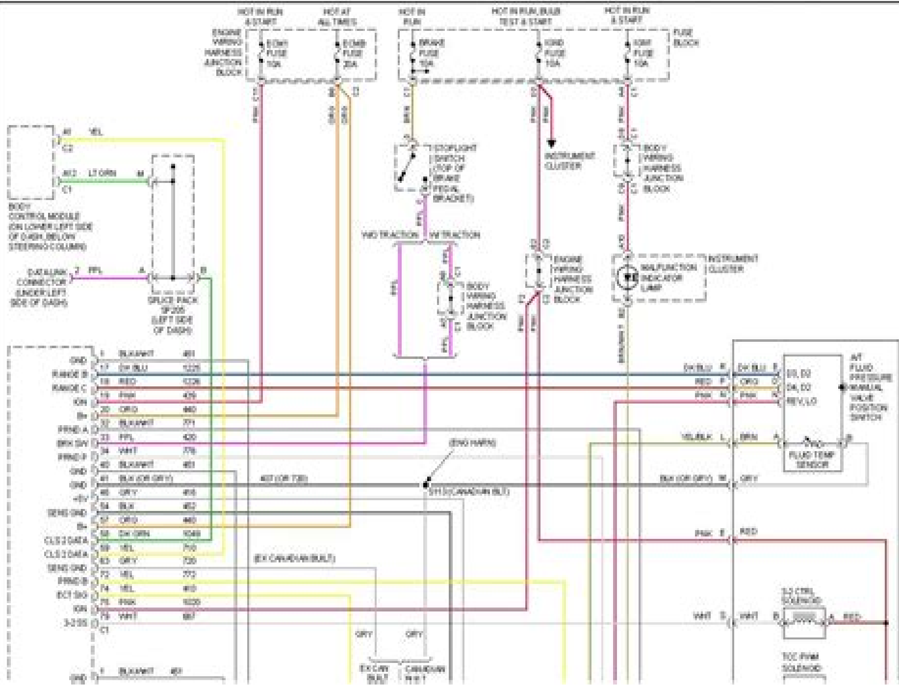
2000 Chevrolet Silverado 1500-Fig. 32: Transmission Control System Wiring Diagram (Sierra, Silverado, Suburban, Tahoe, Yukon)
