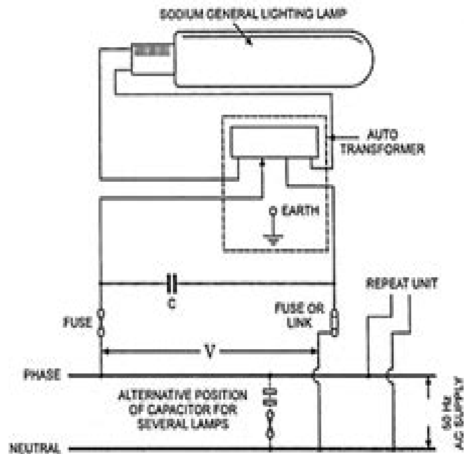
(c) Wiring Diagram
