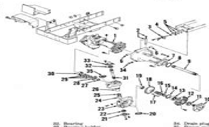
Fig. 7—Exploded view of four-wheel drive front axle assembly available on Model 234.
