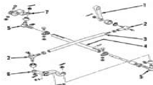
Fig. 6—Exploded view of steering linkage used with adjustable front axle available on Model 234.
