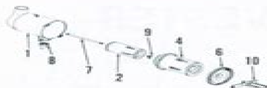
Fig. IH42—Exploded view of typical air cleaner assembly.
