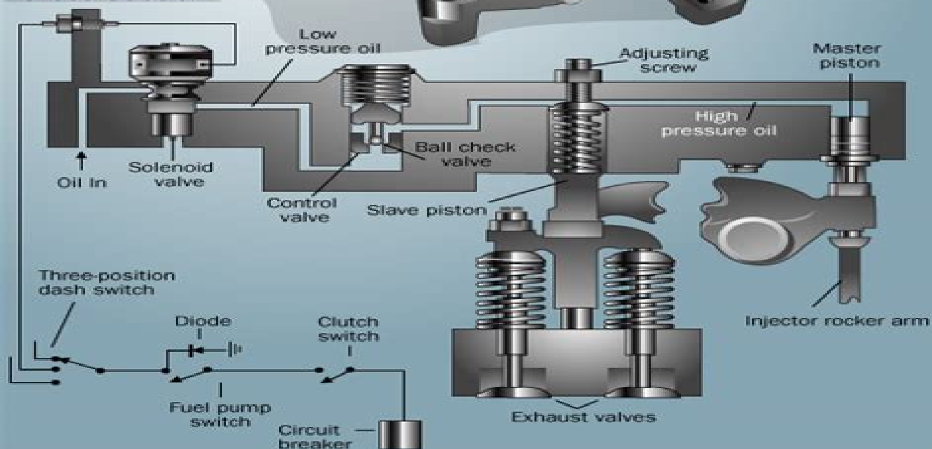
Cross Section
