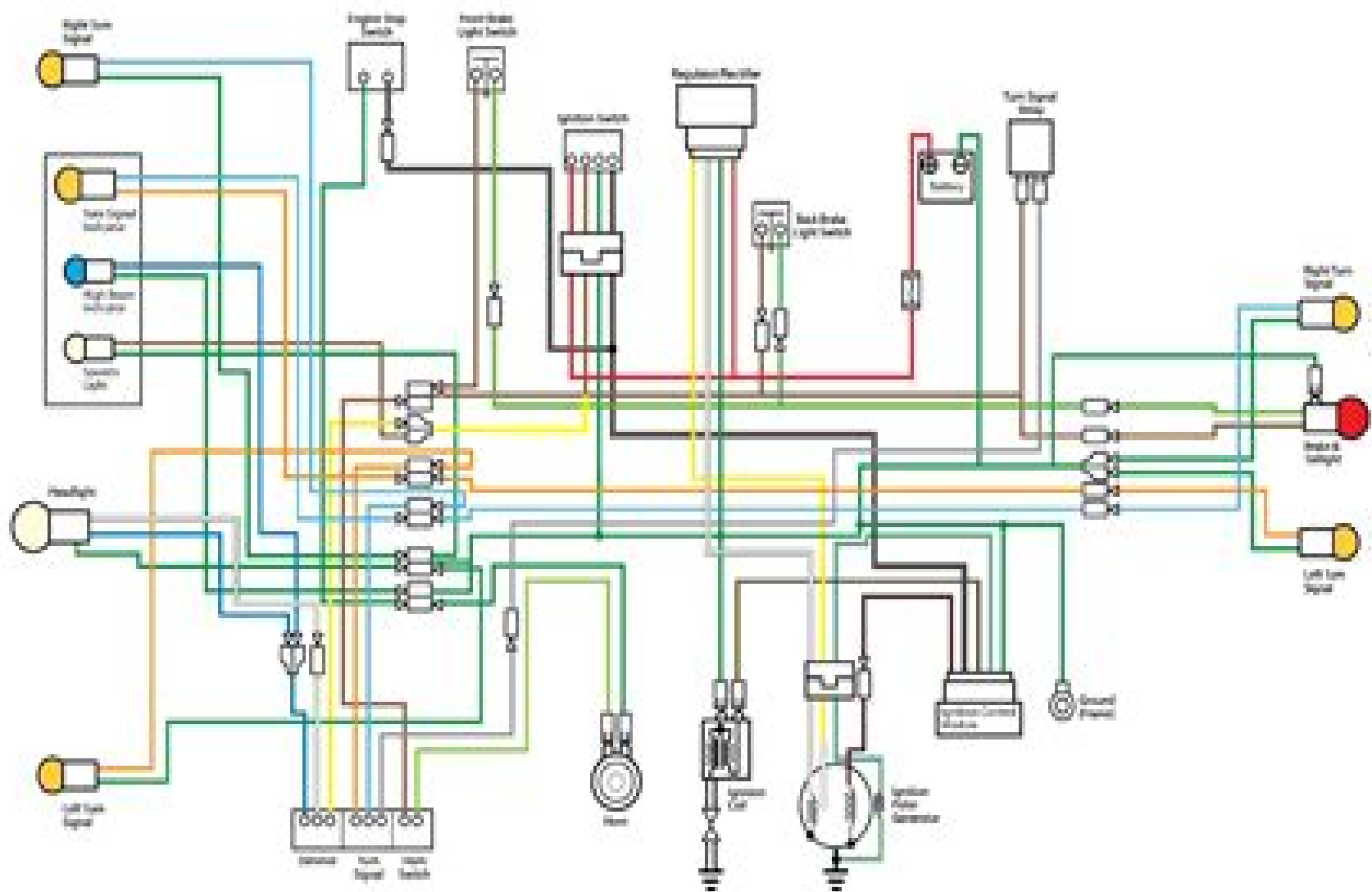
Wiring Diagram
