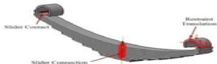
Fig. 2 Boundary condition of MLS
