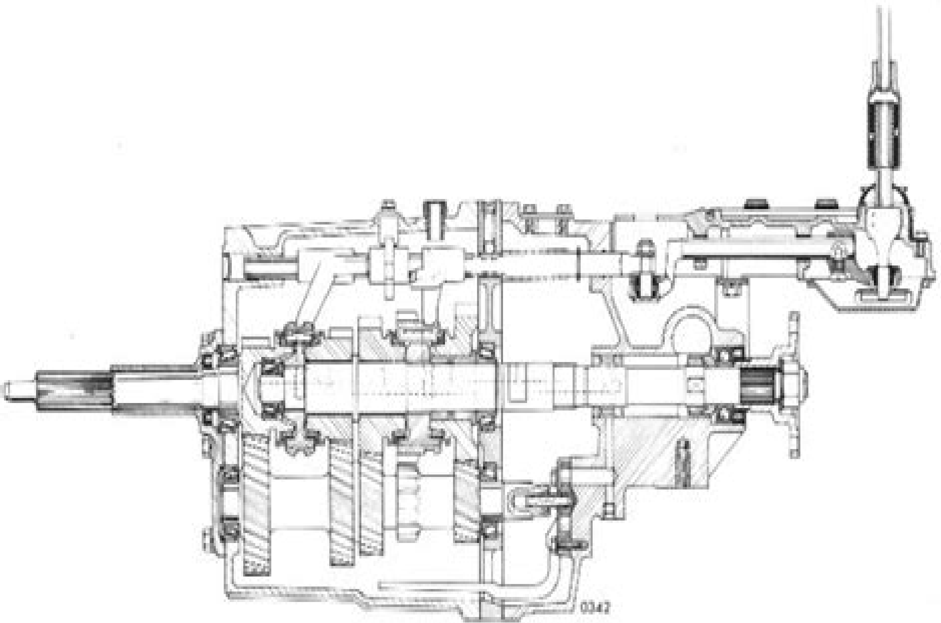
GEARBOX - 4-SPEED
