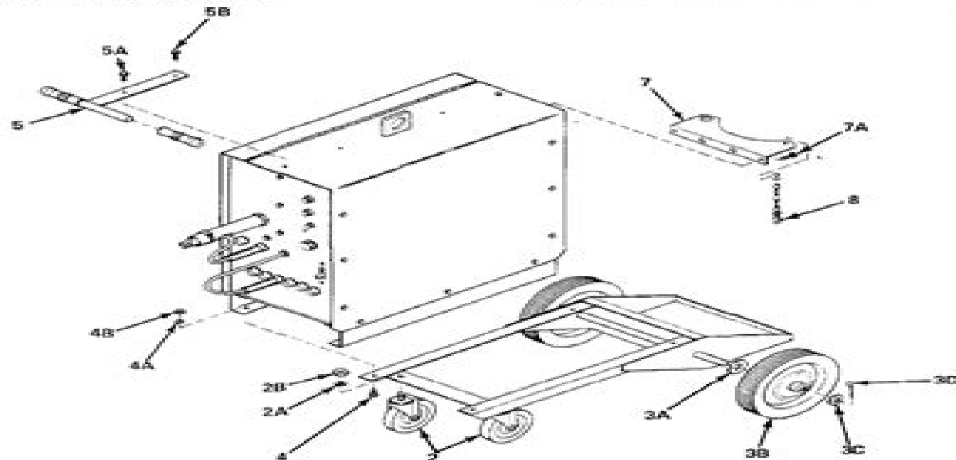
Figure 3-1. Installation of Running Gear
