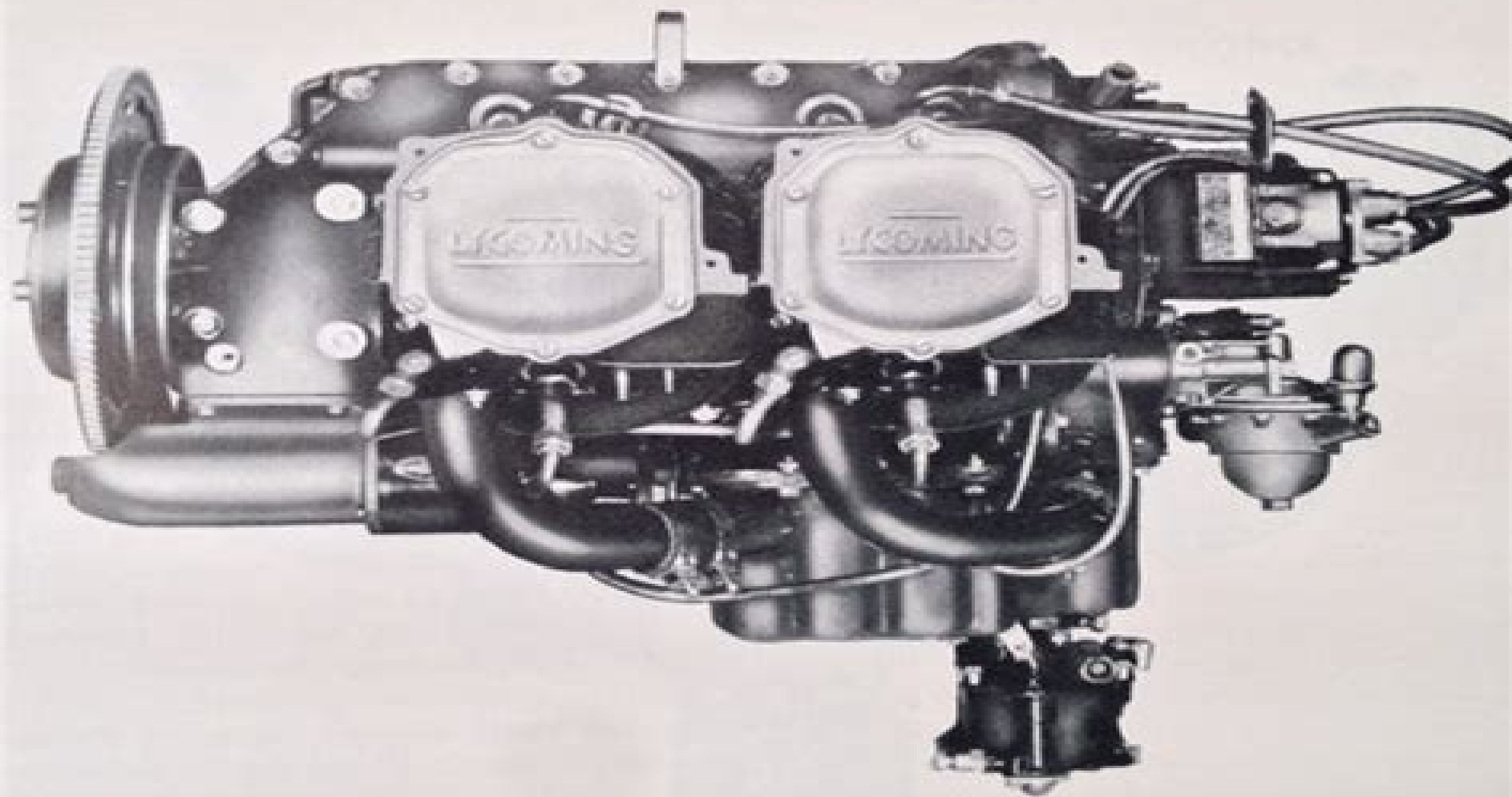
SIDE VIEW
