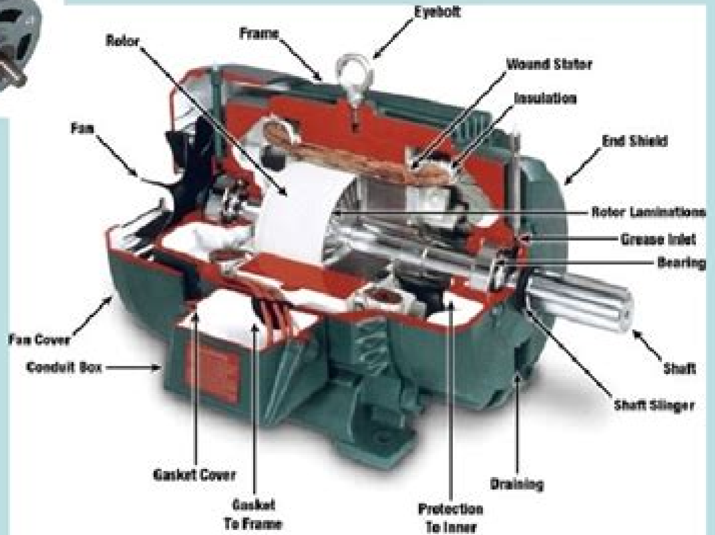
Figure 8 - Motor Construction
