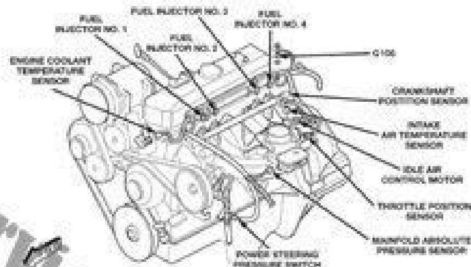
Fig. 8 ENGINE LEFT SIDE 2.4L
