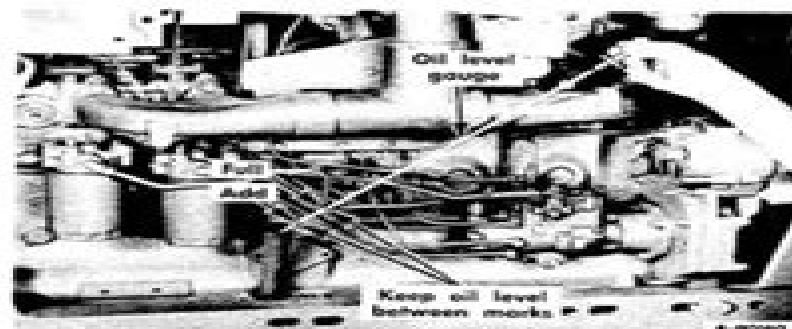
Illustr. 120A Crankcase and oil level gauge. (diesel engine).
