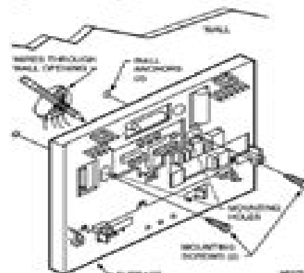
Fig. 2—Mounting subbase on wall.
