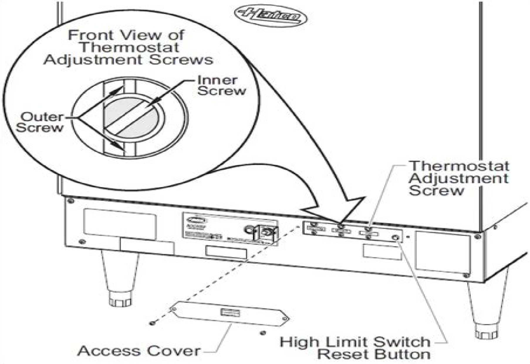
Mechanical Control Thermostat Adjustment and High Temperature Limit Safety Switch (Imperial "S" Model Shown)
