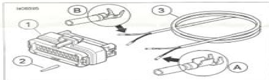
Figure 2. Service Parts, iPod/Navigation Interface Connector Kit
