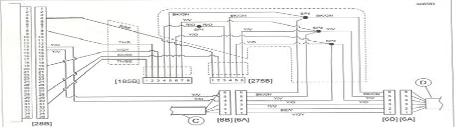
Figure 1. Wiring Diagram, iPod/Navigation Interface Connector Kit
