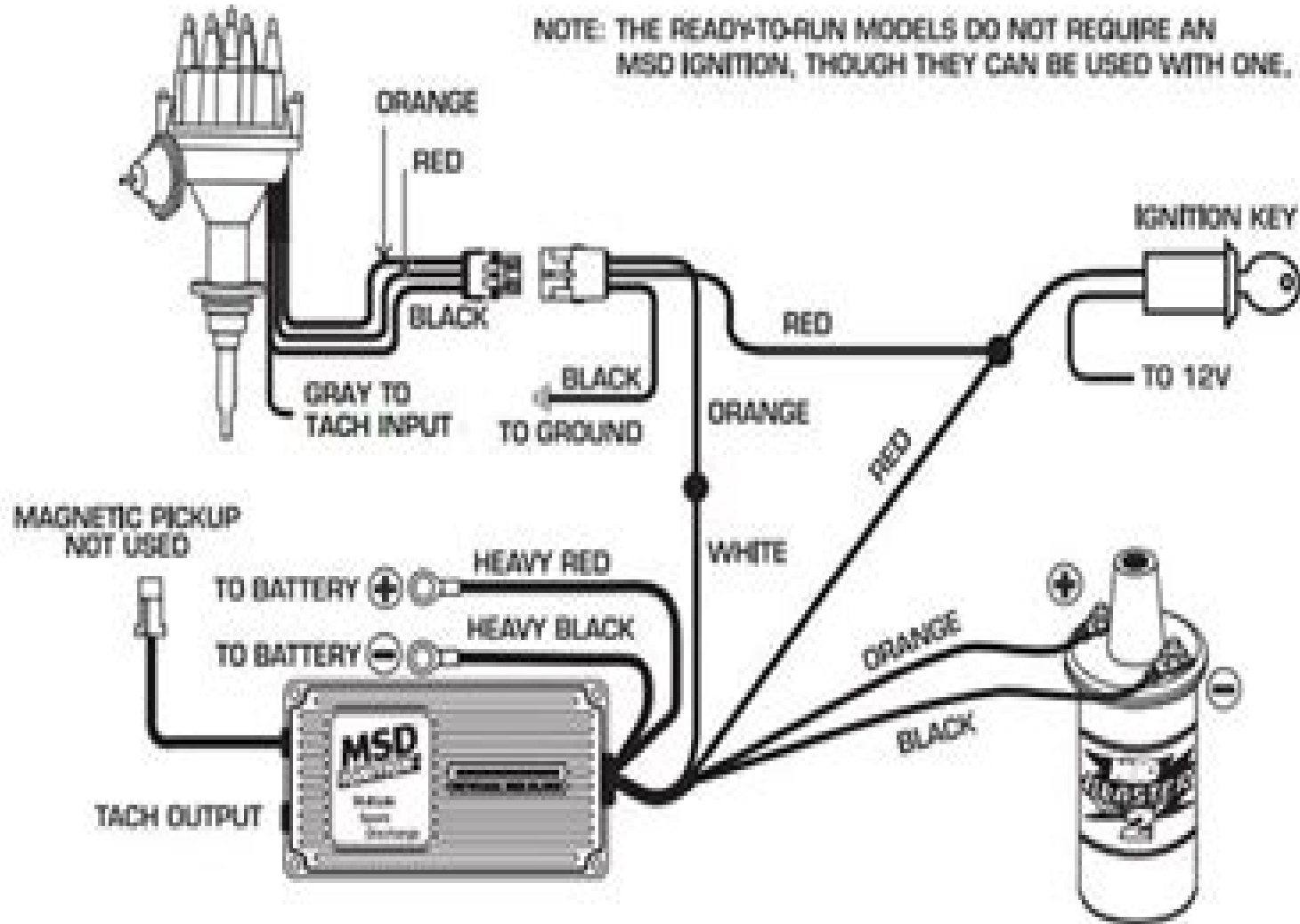
Figure 11 Connecting an MSD Ignition Control.
