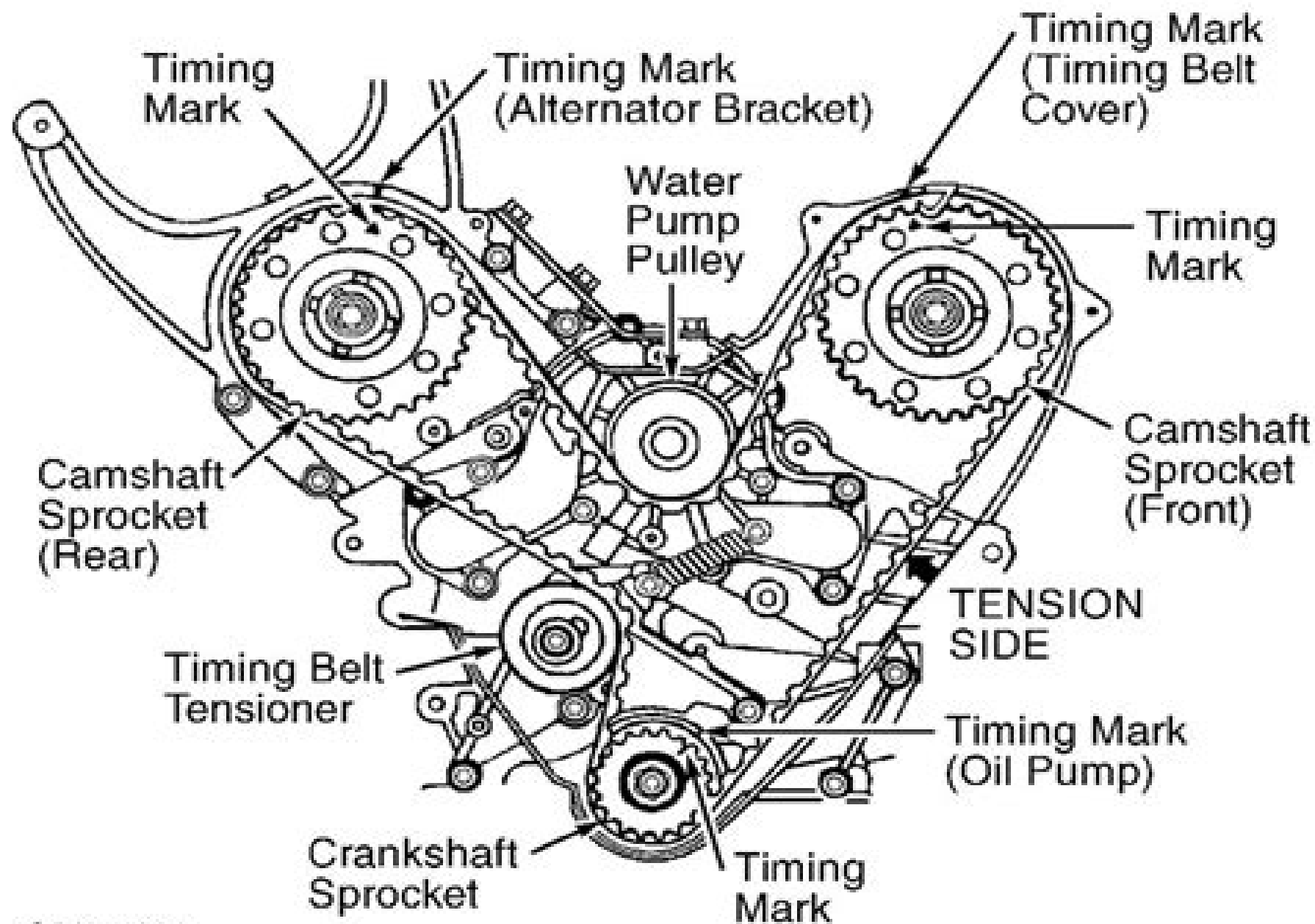
Fig. 3: Locating Timing Belt
