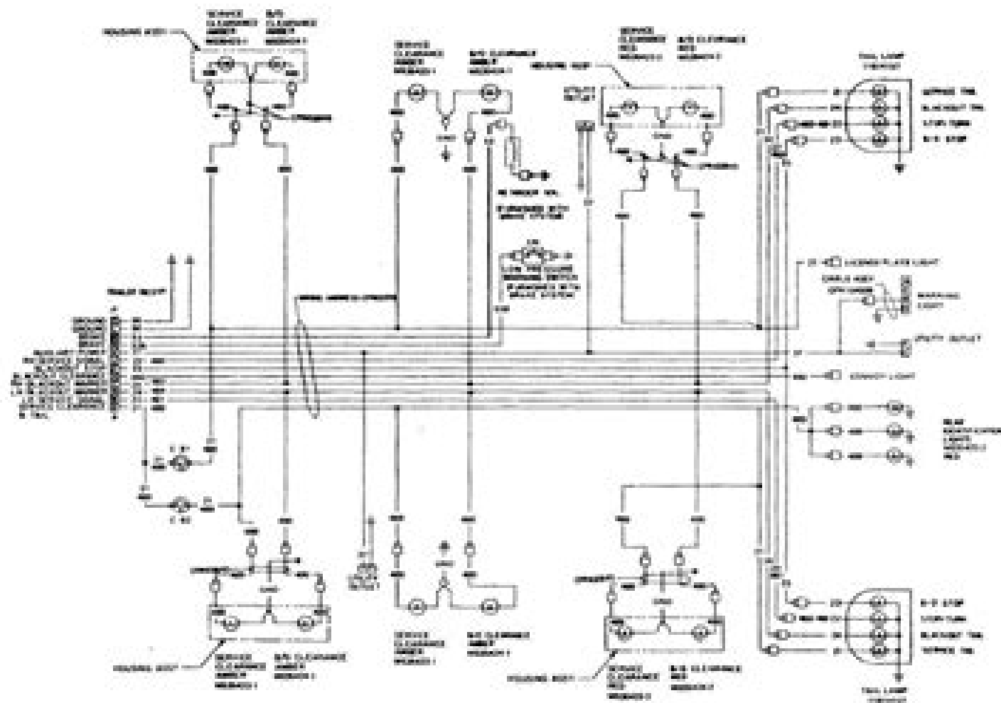
Figure 2d. Wiring schematic diagram (semiconductor No. 1 through 200).
