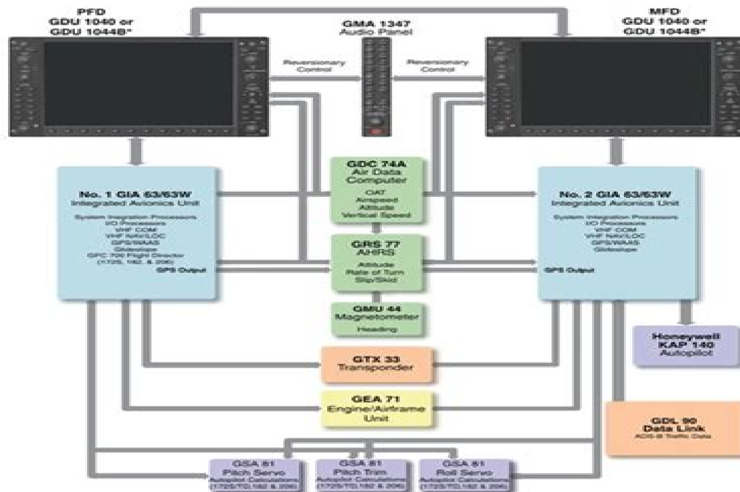
Figure 1-1 Basic G1000 System
