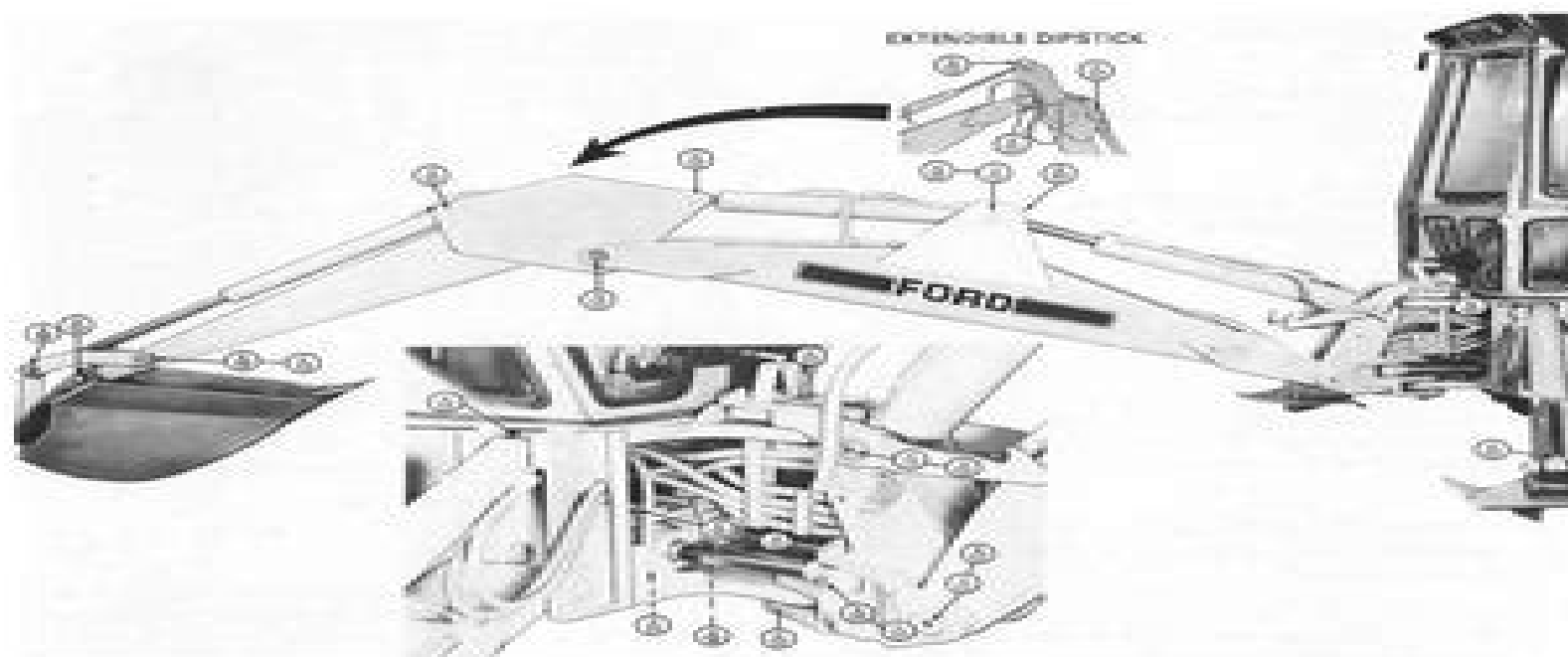
Figure 77 Backhoe Lubrication Points
