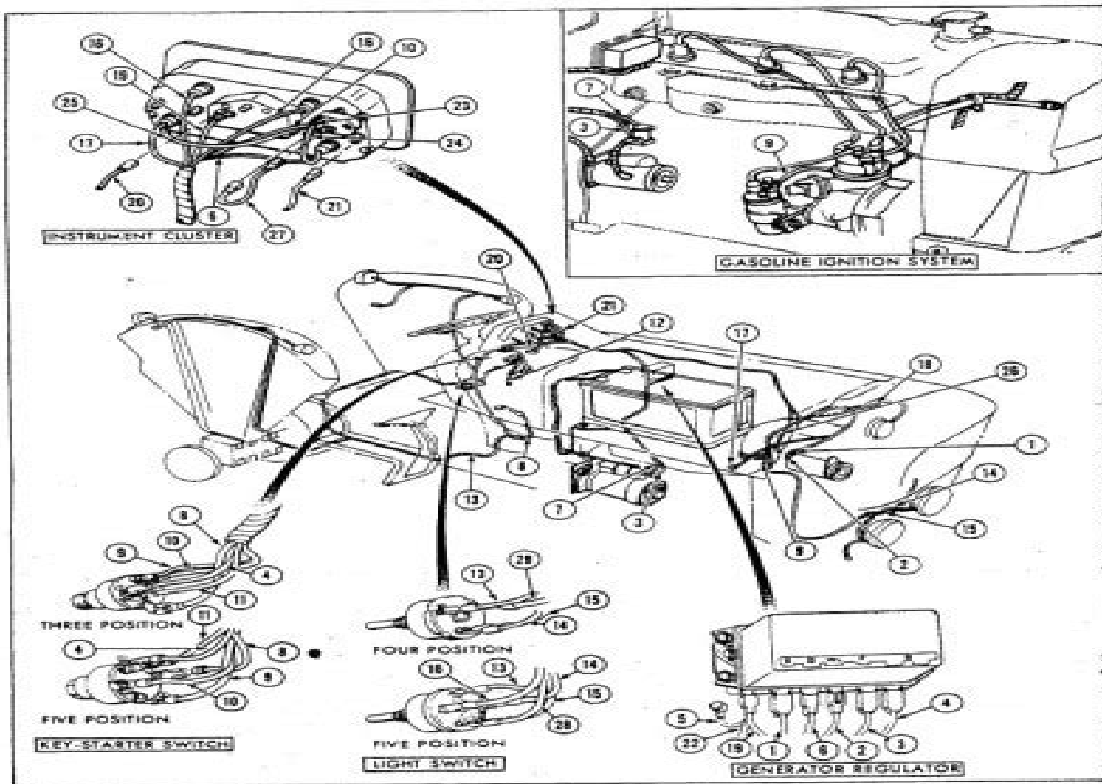
Figure 8 Circuit Descriptions—Tractors with "A" or "B" Prefixed Serial Numbers
