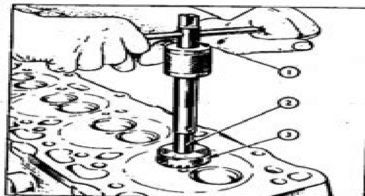
Fig. 4 — Recutting Valve Seats
