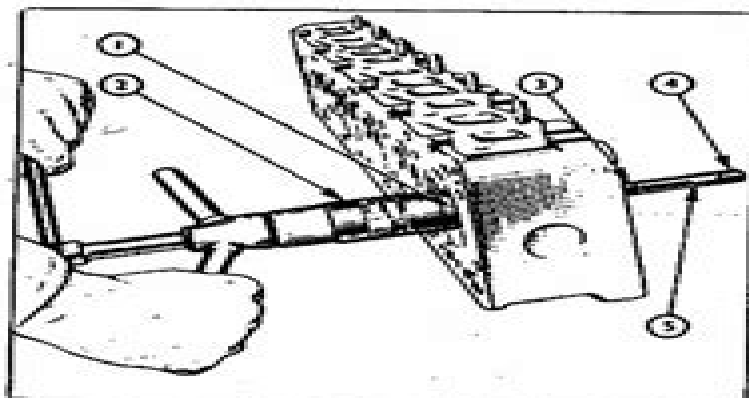
Fig. 3 — Valve Guide Removal
