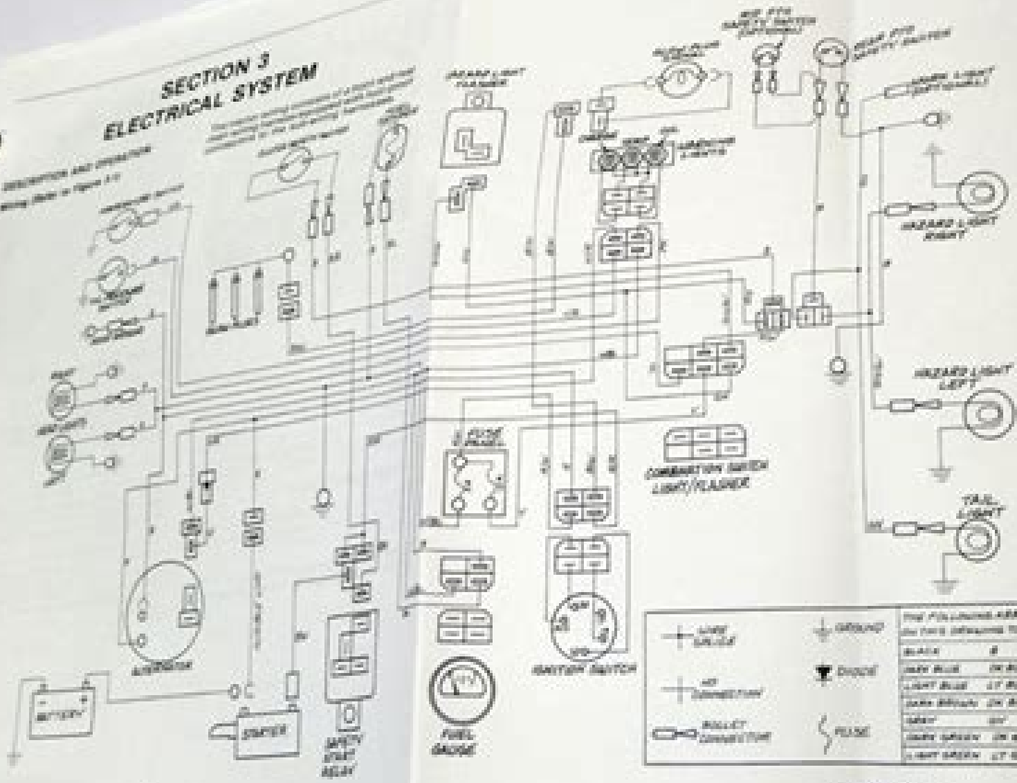
Electrical Diagram
