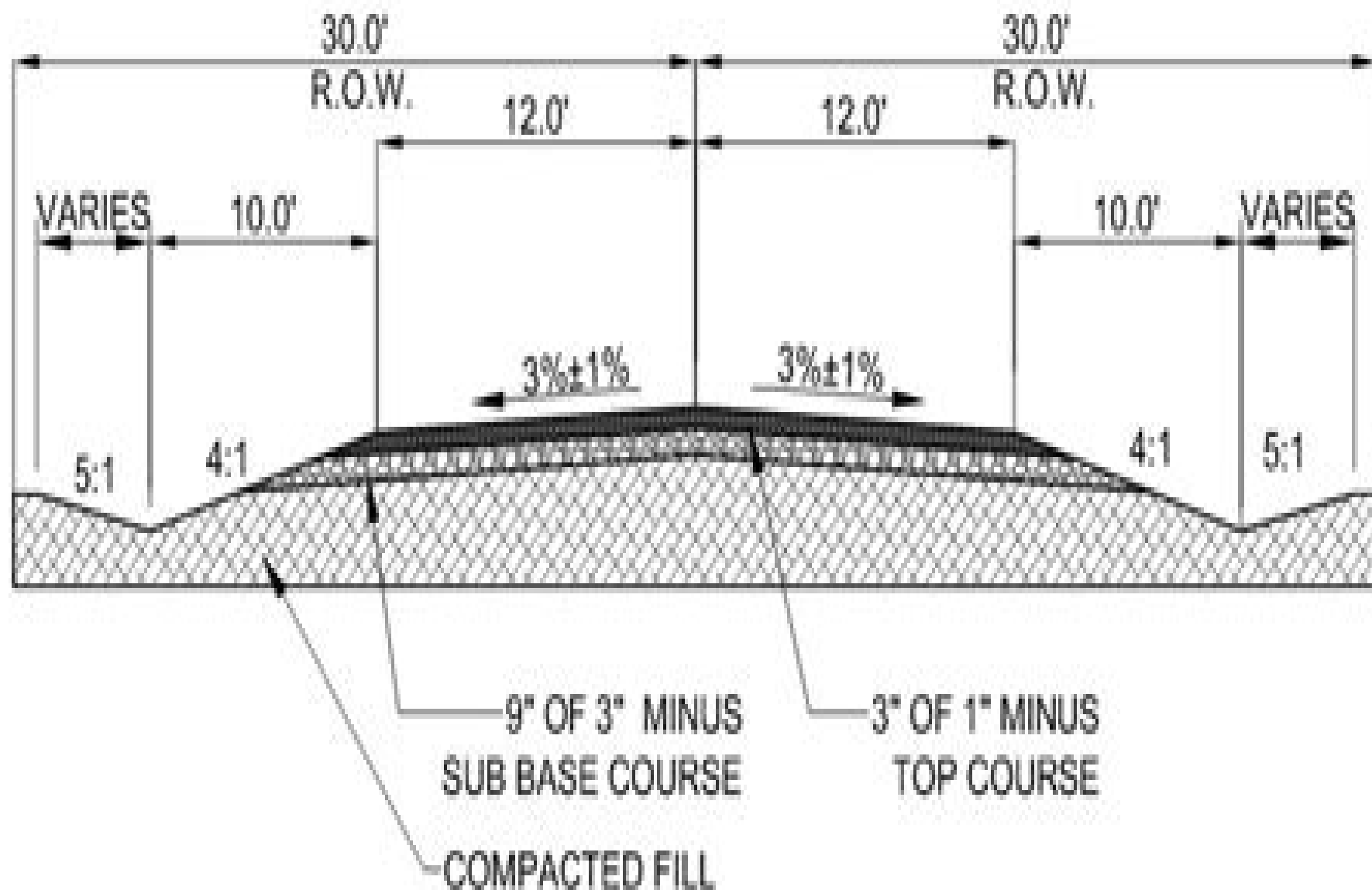
TYPICAL GRAVEL ROAD SECTION
