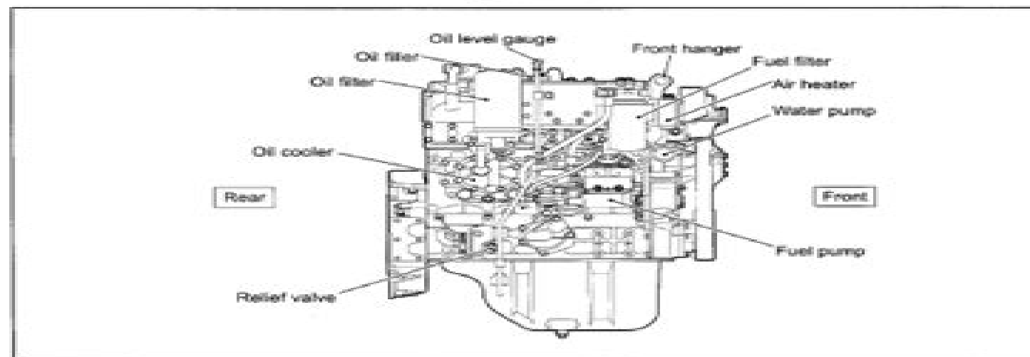
Engine right view
