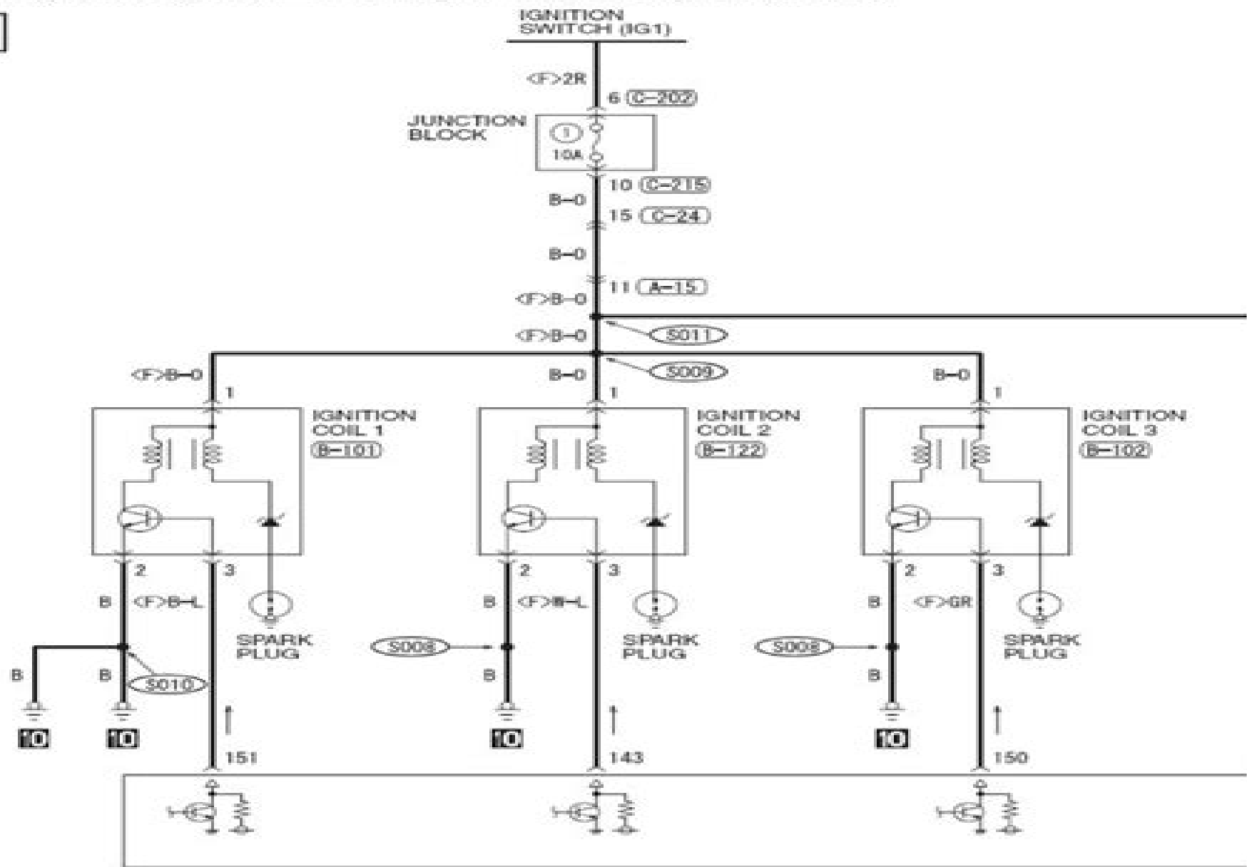
Fig 1: Ignition System - 2.4L Engine Circuit Diagram (1 Of 2)
