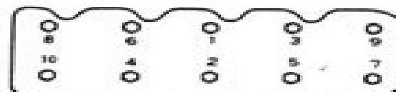
Cylinder head bolt tightening sequence
