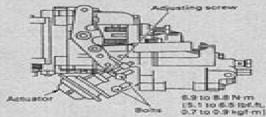
Fig. 13 Idle-up actuator. Manual transmission
