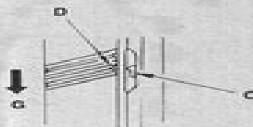
Fig. 12 Timer case & injection pump gear alignment. Except 6D31OAT engines
