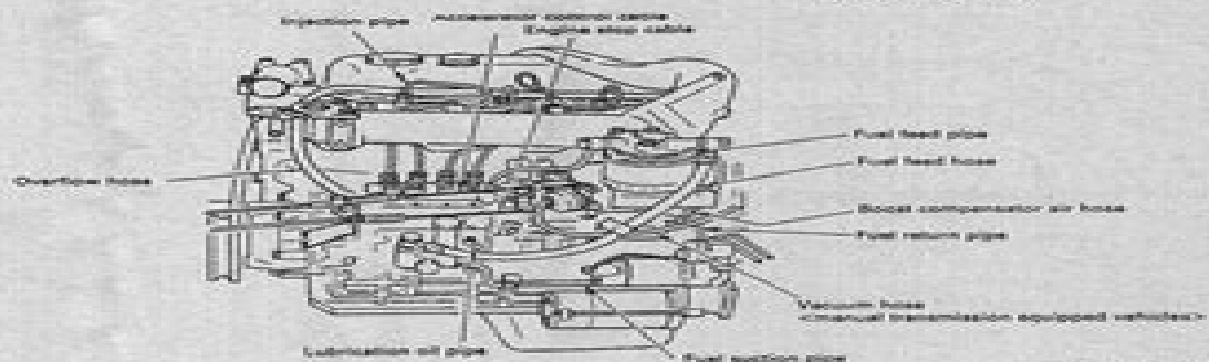
Fig. 15 Fuel Injection system
