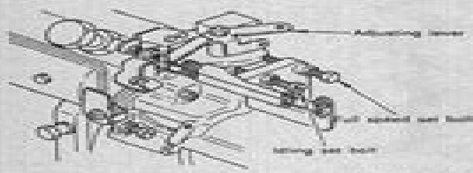
Fig. 14 Minimum & maximum speeds adjustment lever
