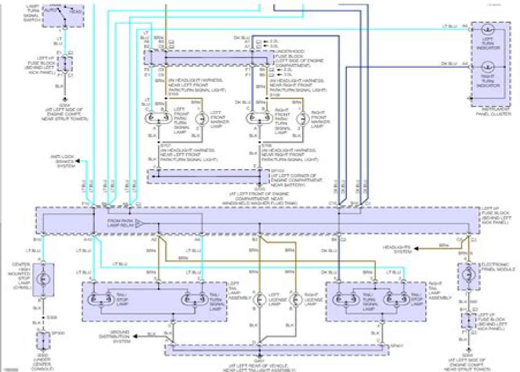
Fig 2: Exterior Lamps Circuit, Sedan
