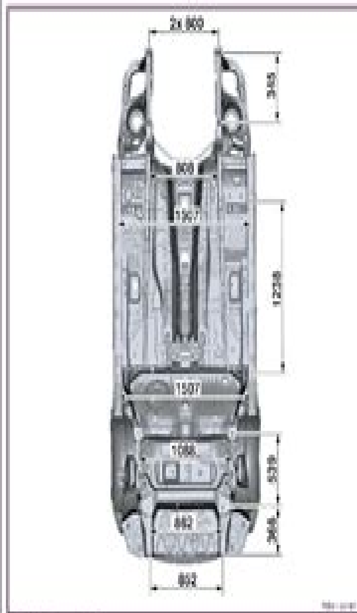
Underbody view 2
