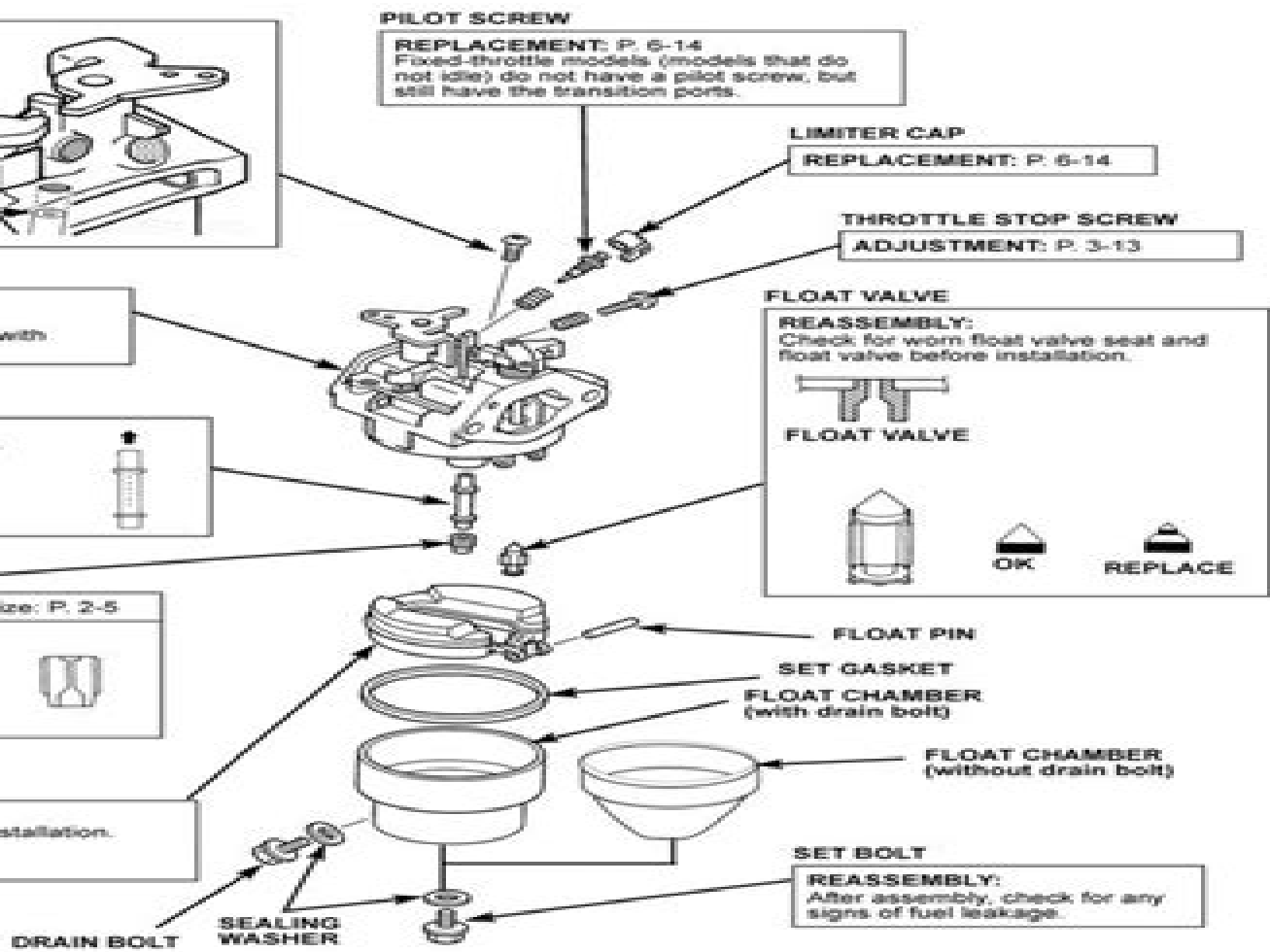
DRAIN BOLT
